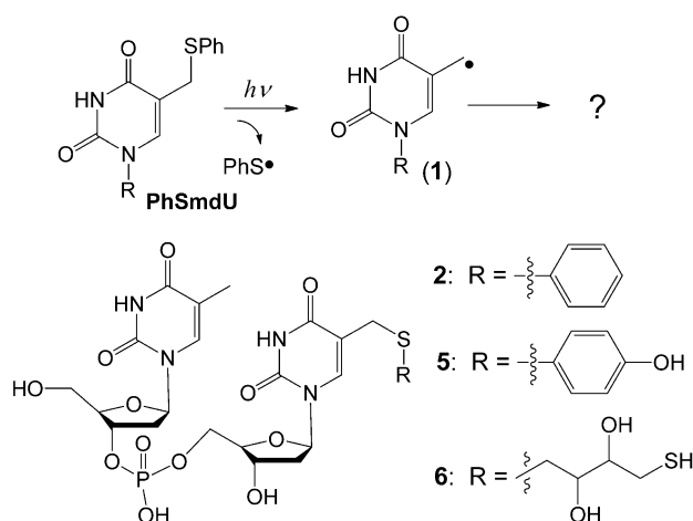
Scheme 1. Generation of 1 by photolytic cleavage of the C–S bond in 5-(phenylthiomethyl)-2'-deoxyuridine (PhSmdU) as well as thiol addition products in the dinucleotide context.
