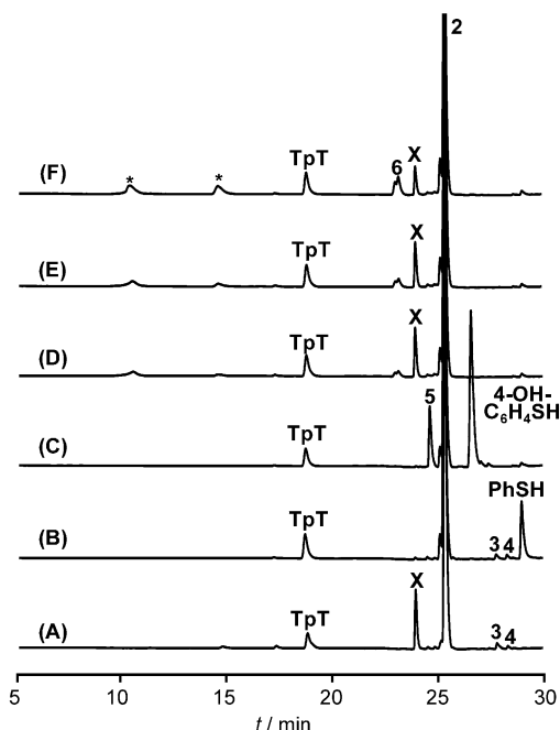
Figure 3. HPLC chromatograph of anaerobic TpPhSmdU ( 2 , 200 \mu M) photoreaction under 254 nm UV light. A) In H_2O ; B) with 1 mM PhSH; C) with 1 mM 4-OH- C_6H_4 SH; D) with 1 mM DTT; E) with 10 mM DTT; and F) with 40 mM DTT. As the DTT utilized was a DL mixture, the resulting adducts 6 were a mixture as well, as indicated by the doublet peak in the HPLC chromatograph. The two peaks marked by * correspond to DTT and DTT disulfide, respectively, which already exist in the DTT used. [13]
