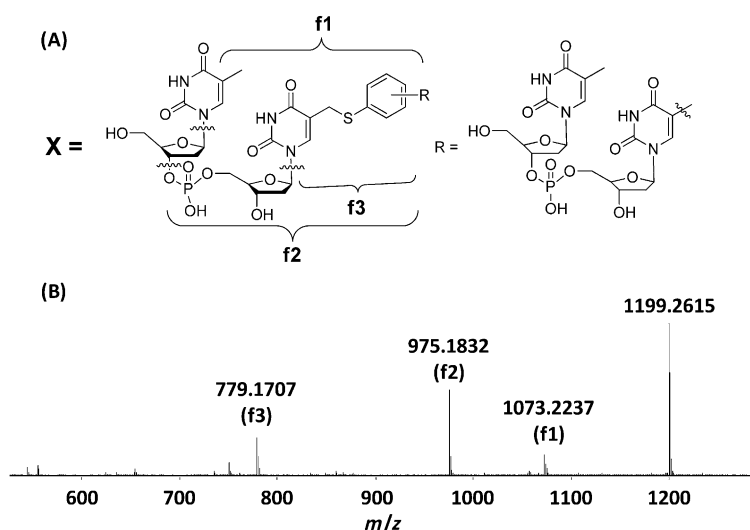
Figure 2. A) Proposed structure of product X, suggesting that a TpT moiety is added to the phenyl ring of -SPh. B) LC-MS/MS analysis of ion [\text{X} + \text{H}]^+ at 1199.26. The structures of the three fragmentation ions (f1, f2, and f3) are indicated in (a).
