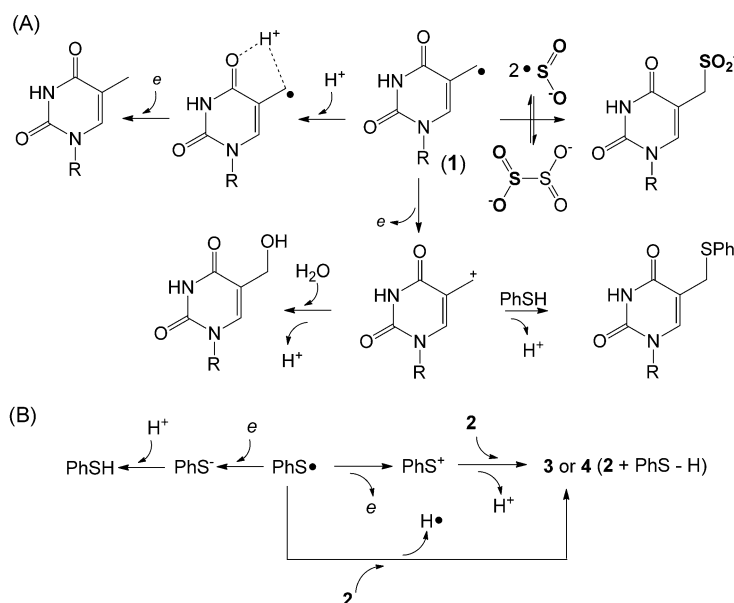
Scheme 3. Oxidation and reduction reactions of 1 and \text{PhS}^\bullet .
