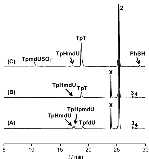
Figure 1. HPLC chromatograph of TpPhSmdU ( 2 , 200 \mu M) photoreaction under 254 nm UV light. A) In \text{H}_2\text{O} in air; B) in degassed \text{H}_2\text{O} in a Coy anaerobic chamber; C) in degassed \text{H}_2\text{O} in a Coy anaerobic chamber and supplemented by 1 mM sodium dithionite.
