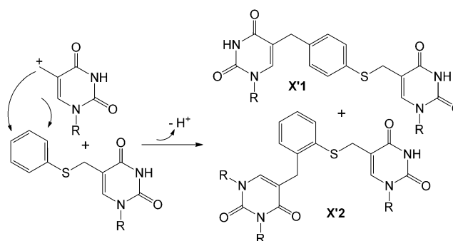
Scheme 2. Addition of the thymine methyl cation to the para position of the phenyl ring in X'1 and to the ortho position in X'2.
